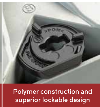
Twist-lock anchors securely retain concrete in lid
